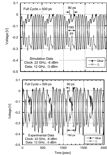
Figure 9. Top graph shows simulated flip-flop outputs; bottom graph shows measured flip-flop outputs, for a 22 GHz clock frequency.
