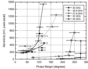
Figure 7. Above graph shows measured data input voltage vs. measured phase margin for the frequency range of 20-30 GHz.
