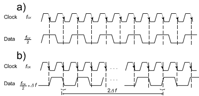
Figure 8. a) Timing diagram illustrating clock and data timing for divide-by-2 operation; b) Electronic phase-shifting timing diagram, where data rate is f_{CK}/2 + Df , showing how the additional periodicity of the outputs will be 2Df .
