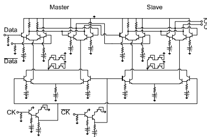
Figure 4. Schematic diagram of master-slave D-flip-flop circuit, showing all on-chip circuitry.
