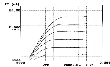
Figure 2. DC I-V characteristics of a dual-emitter HBT, having an emitter area of 20 mm 2 . Base current, I_b , was applied in steps of 400 nA.
