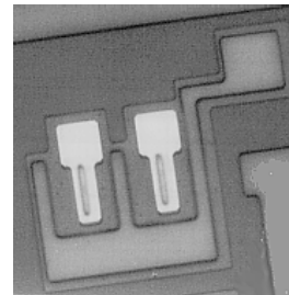
Figure 1. Micrograph showing a pair of InGaAs HBT's sharing a common collector. The single emitters are 1 x 10 mm 2 stripes.
