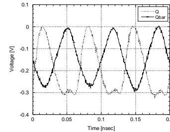
Figure 6. The graph shows a plot of the two flip-flop outputs, Q and Qbar , for a 30 GHz clock input frequency and a 30 Gb/sec input data rate, for an input data voltage of 600 mVp-p.
